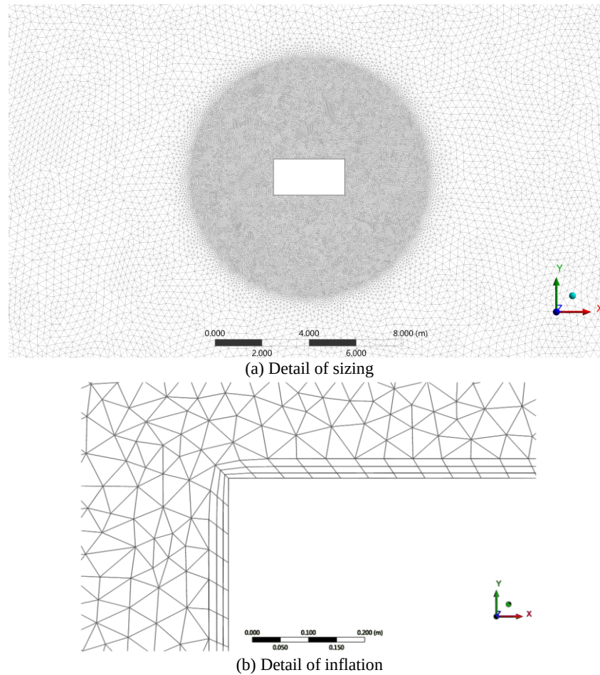
Figure 2. Mesh for initial stage. Source: the authors.
