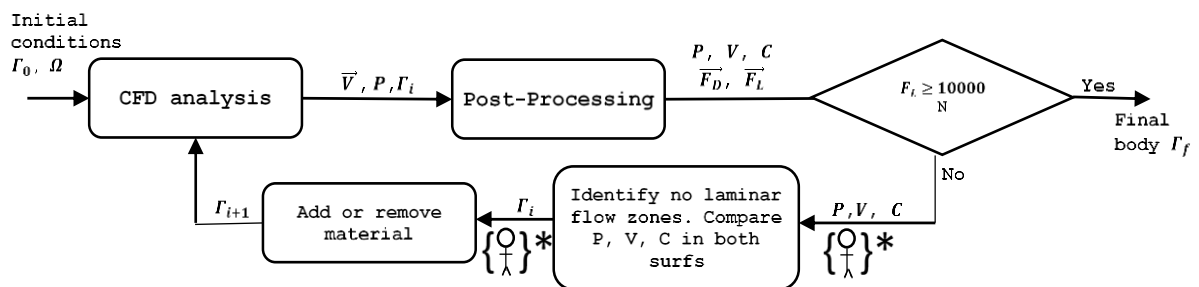
Figure 3. Evolution process diagram. *: Human iterative interaction. Source: the authors.
