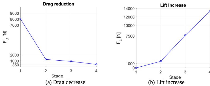
Figure 5. Drag and Lift evolution. Source: the authors.
