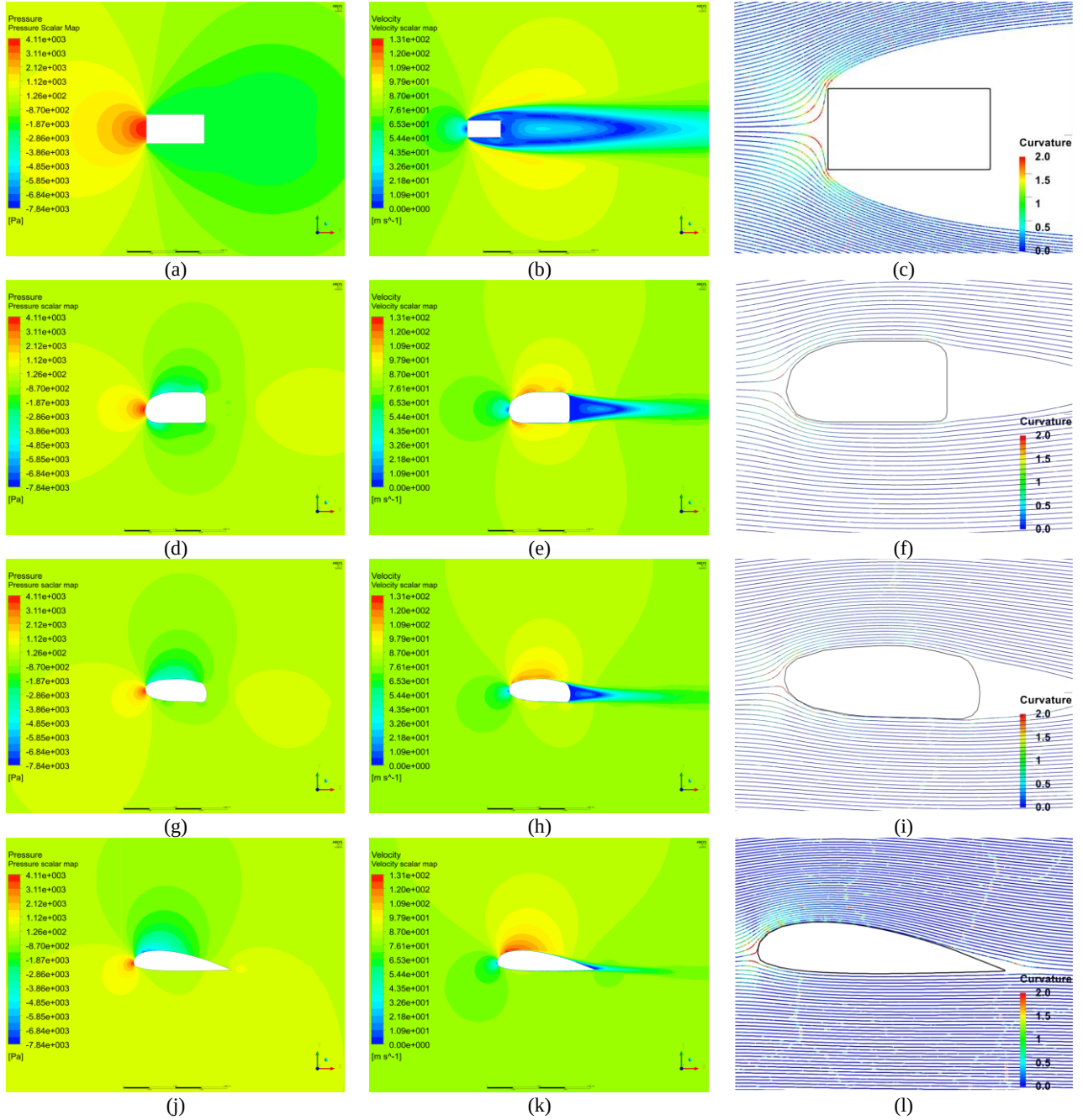
Figure 4. Evolution scalar maps of velocity, pressure and streamlines. Source: the authors.
