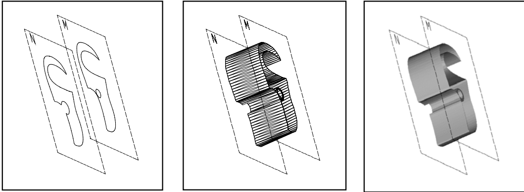
Fig. 9 - Addition of 1-handle. Croissant – Donut transition.
