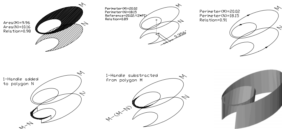
Fig. 8 - Algorithm to infer relations between set of contours in levels L_j and L_{j+1} .
