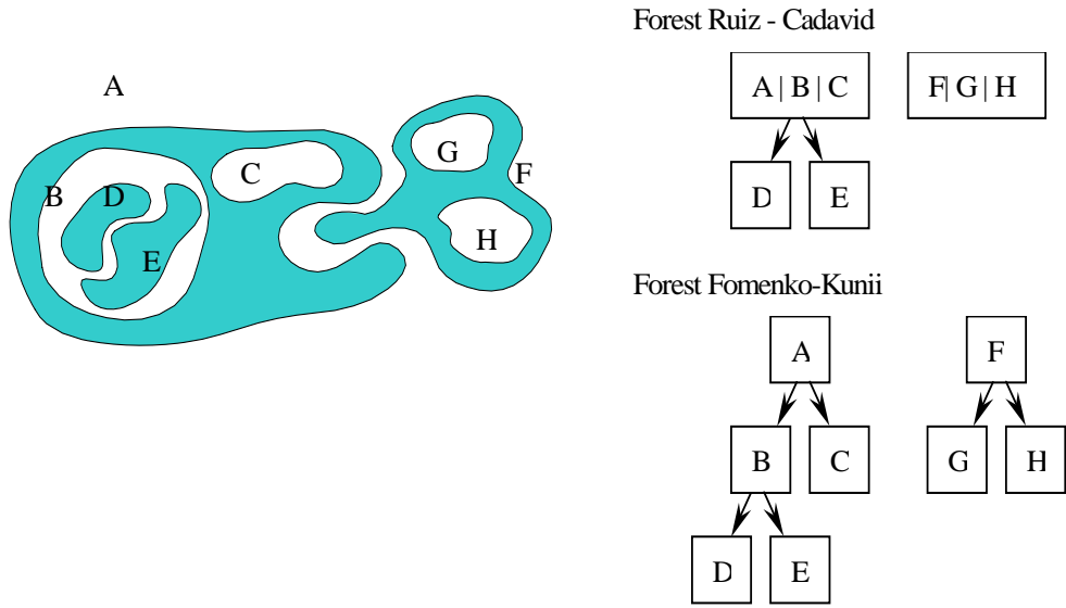
Fig. 5 - Forest structures to represent cross cuts of 2-mainfold
